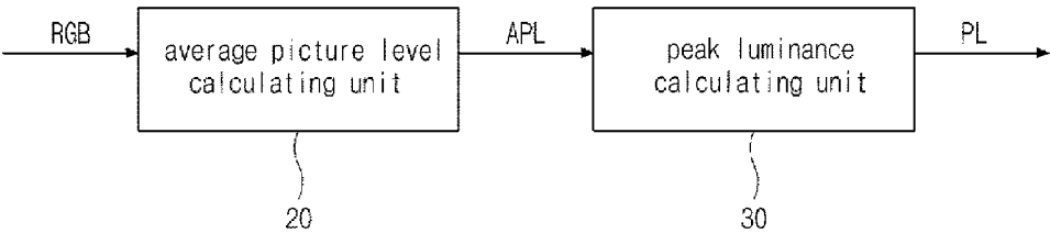
FIG. 2 Related Art
